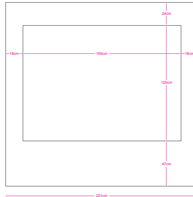
2m Window Wall
