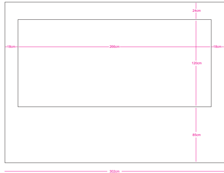
3m Window Wall
